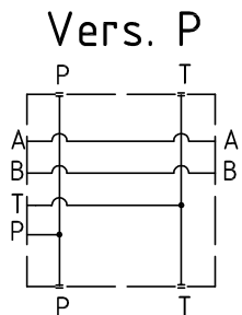
collegamento parallelo parallel connection
